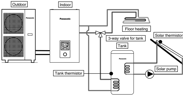
Tank + Solar connection
