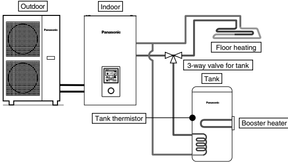
DHW (Domestic Hot Water) Tank connection
